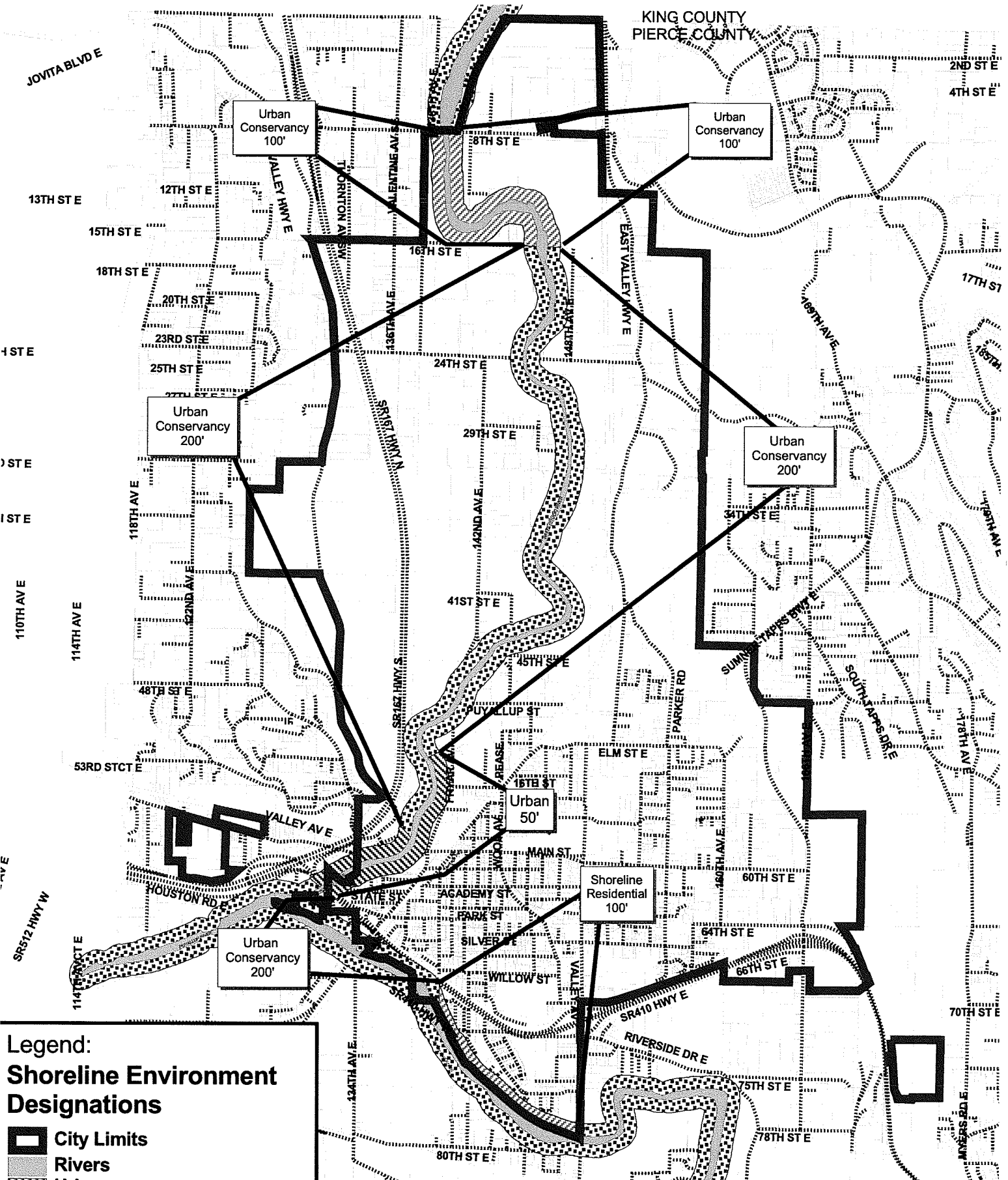
Figure 4-1 Sumner Shoreline Environment Designations Sumner, Washington
